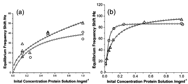
Figure 3. Langmuir adsorption isotherms of (a) BSA and (b) fibrinogen onto \text{CH}_3 - (O) and \text{OH} - ( \Delta ) terminated surfaces.
